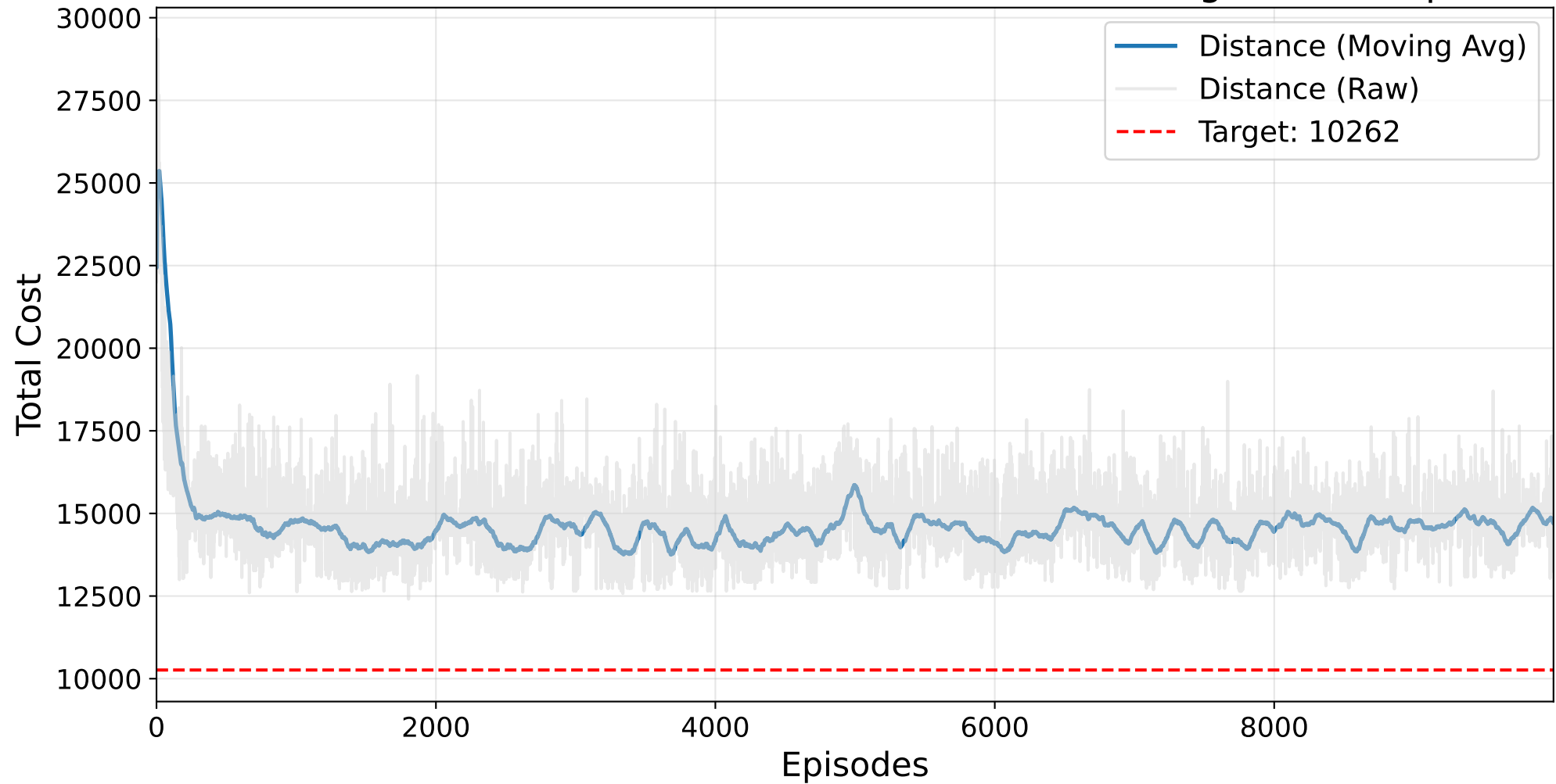
Final HYPERBAND TPE Masked AutoRL-SOP Training - ft53.3.sop
